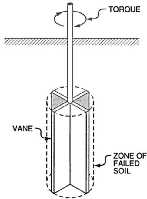
Figure 11: Field Vane Shear Test (Selig and Waters, 1994)
