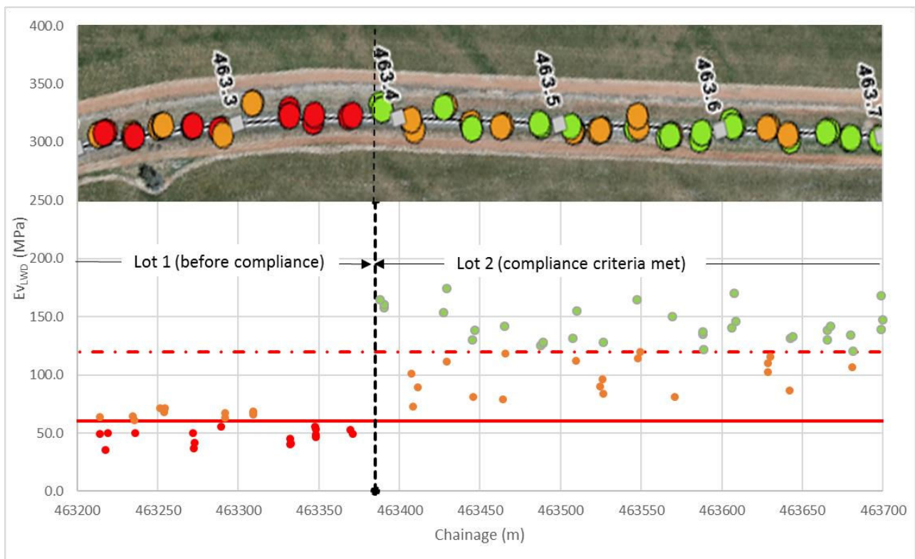
Figure 10: Geospatial reporting of LWD results
