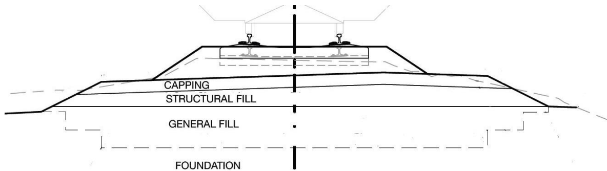
Figure 1: Summary of material designation in accordance with ARTC ETC-08-03
