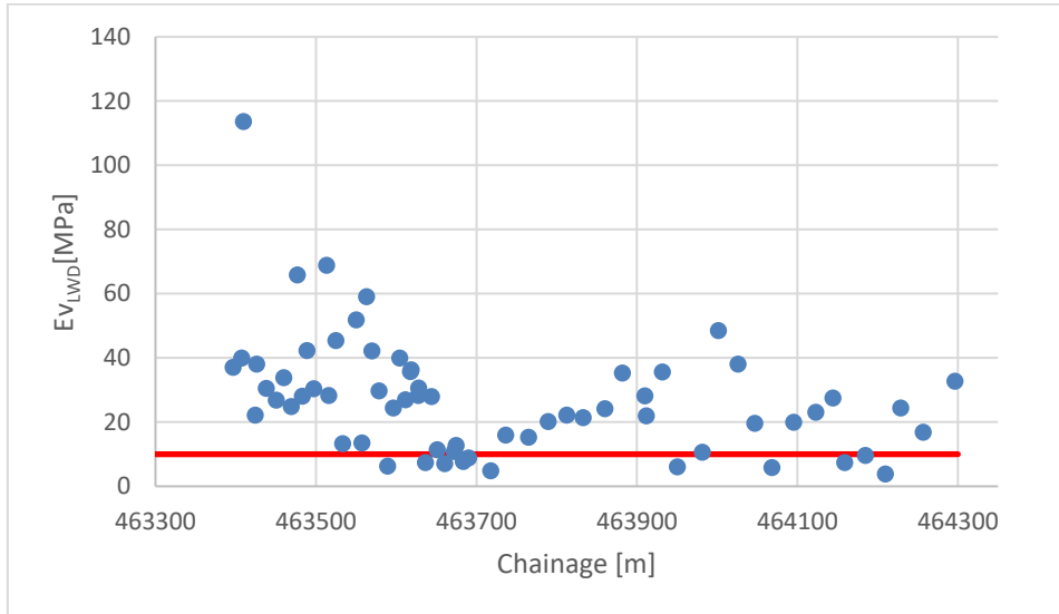
Figure 6: E_{V_{LWD}} plotted with published (10MPa, red solid line) on foundation level for CH463300 to 464300
