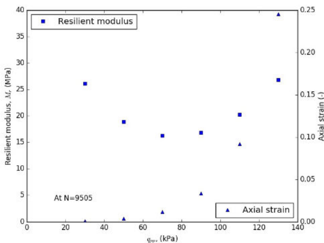
Figure 3: Cyclic triaxial laboratory results, graph shows end of stage resilient modulus versus target deviatoric stress amplitude
