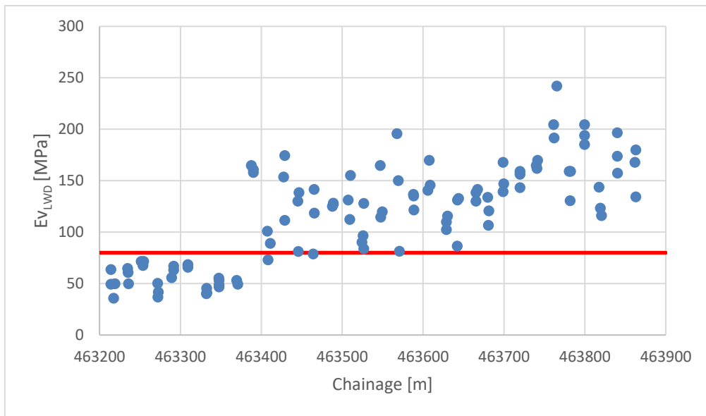
Figure 9: E_{VLWD} plotted with published data (red solid line) for capping from CH463200 and CH463900 (Lot 1 and Lot 2)
