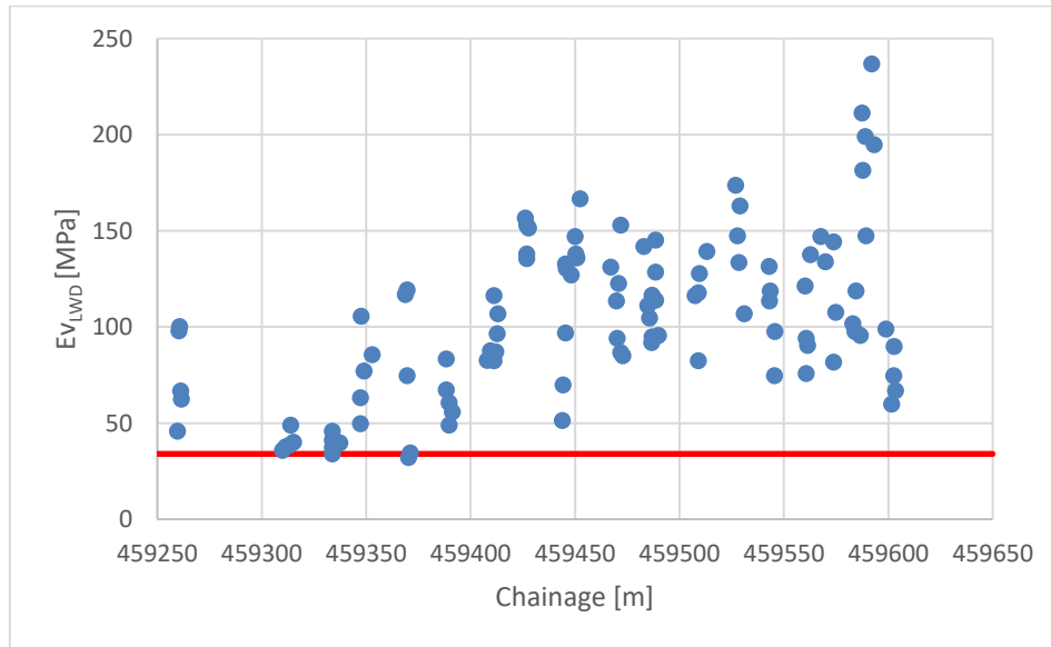
Figure 8: E_{VLWD} plotted with published data (red solid line) for structural fill from CH459250 to CH459650
