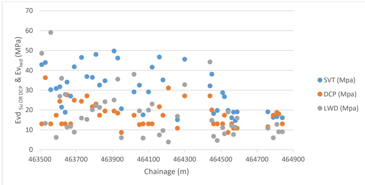
Figure 5: E_{V_{LWD}} and E_{vd_{Su \& DCP}} on foundation level from chainage CH463500 and CH464900
