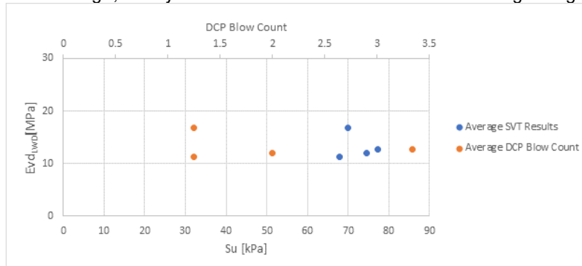
Figure 4: E_{VLD} where SVT compliance testing S_u ranged between 40 and 80kPa
