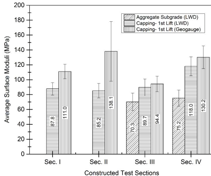
Figure 4: Surface measured moduli on aggregate subgrade and capping layers
