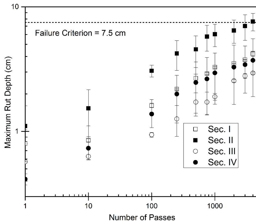
Figure 5: Rutting accumulations with number of load applications for Sections I through IV
