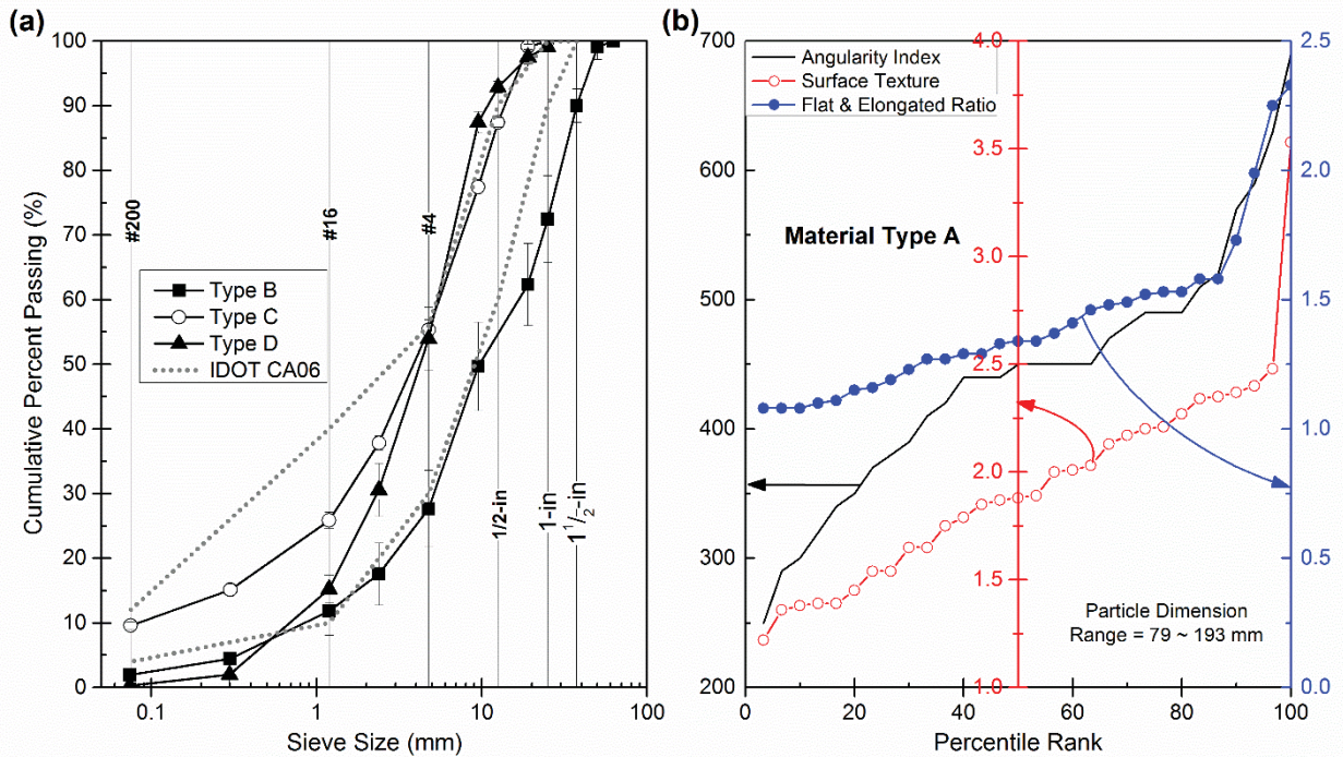
Figure 2: (a) Particle size distributions of Type B, C and D aggregates; (b) Aggregate imaging based shape indices of Type A aggregates
