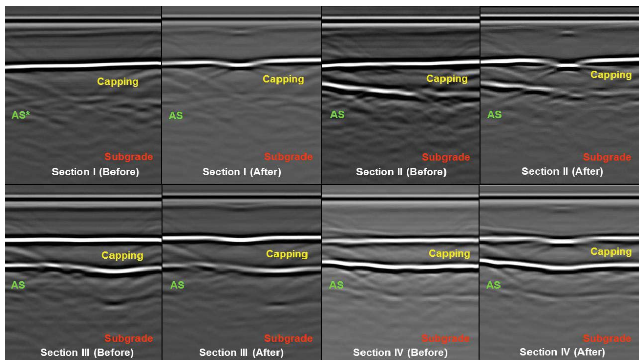
Figure 6: GPR scans of the constructed test sections (AS* = Aggregate Subgrade)
