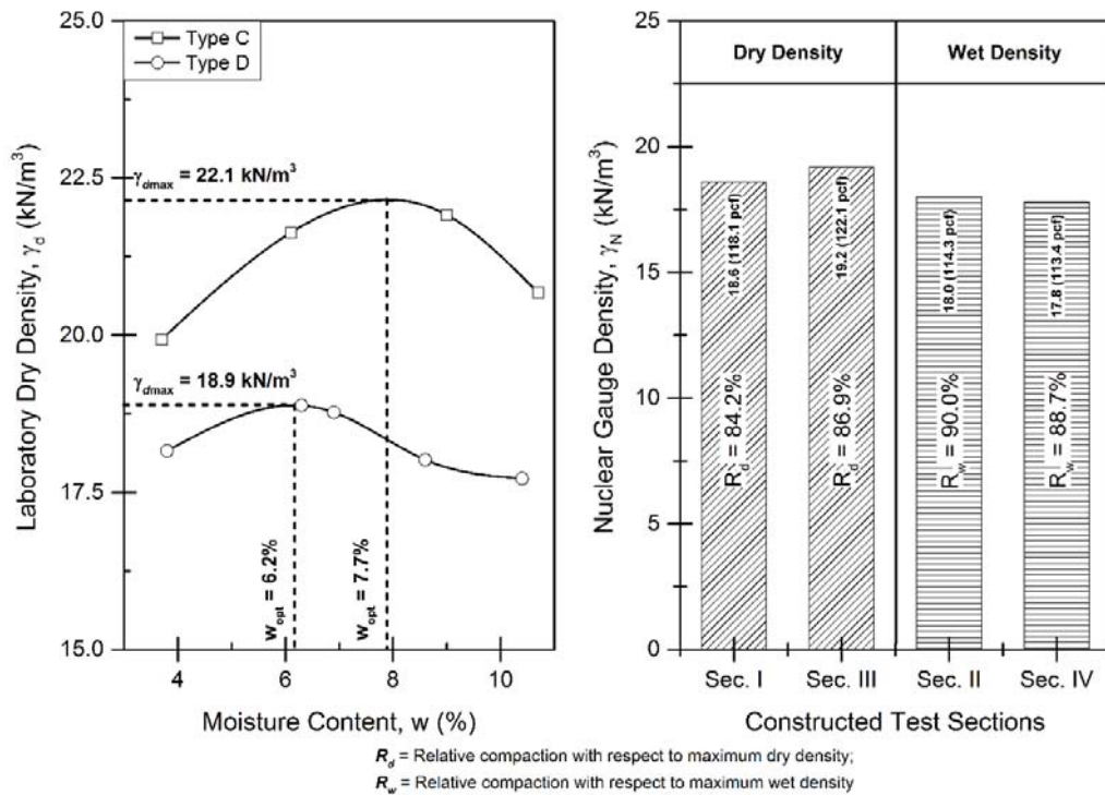
Figure 3: Laboratory standard Proctor and field compaction characteristics of capping materials
