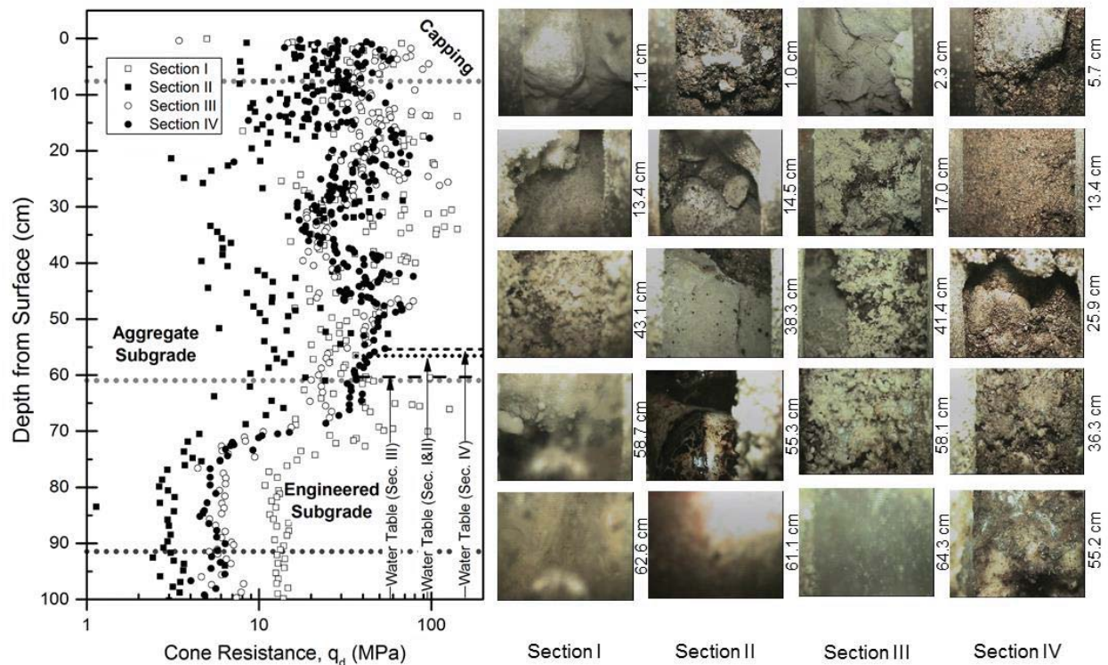
Figure 7: Cone resistance from variable energy penetration tests with geo-endoscopic images
