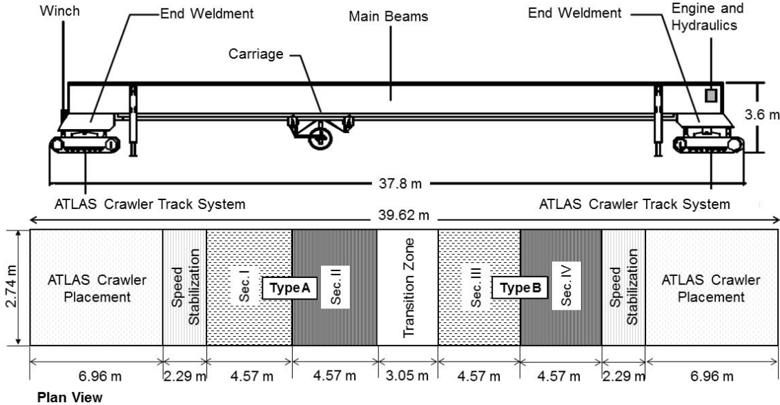
Figure 1: Plan view of the constructed test sections
