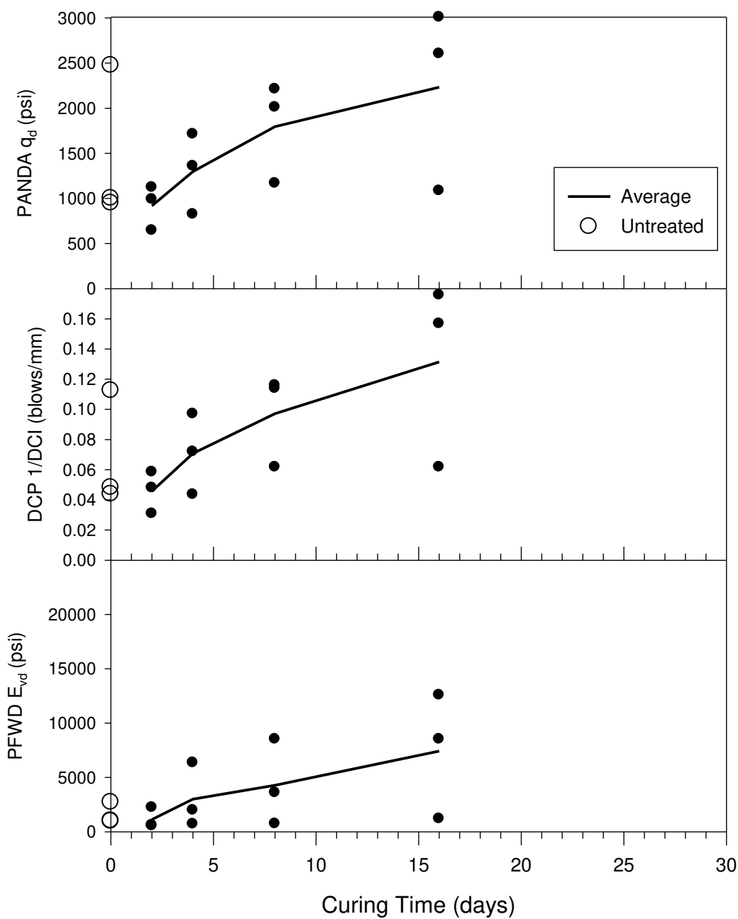
Figure 35: Results of Field Testing at Site #5, US 81
