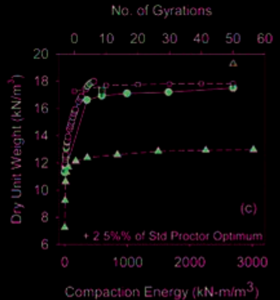
Comparison of relationship between dry unit weight and impact, static, and vibratory compaction energy, and number of gyrations for mixed glacial till at (a) dry of optimum, (b) optimum, and (c) wet of optimum moisture content from standard Proctor test.
