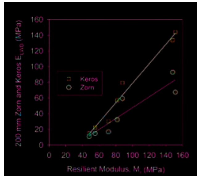
Comparison of 200 mm Zorn, Keros E_{LWD} , and Resilient Modulus ( M_r )
