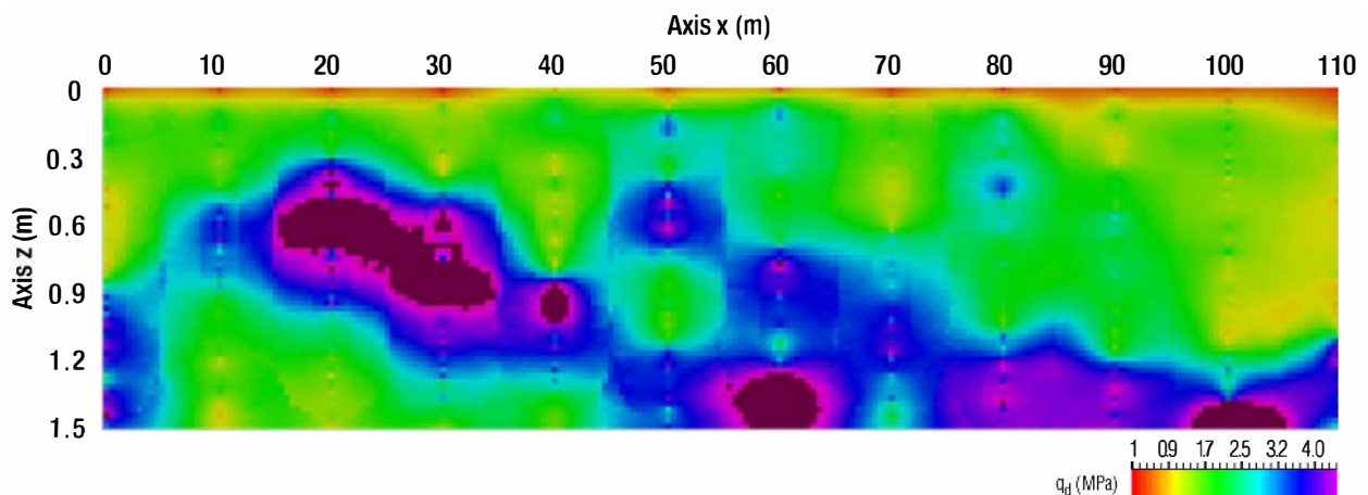
Figure 10. OK estimation of q_d . xz -plane longitudinal profile. Survey grid: First third, near the embankment dam crest.
