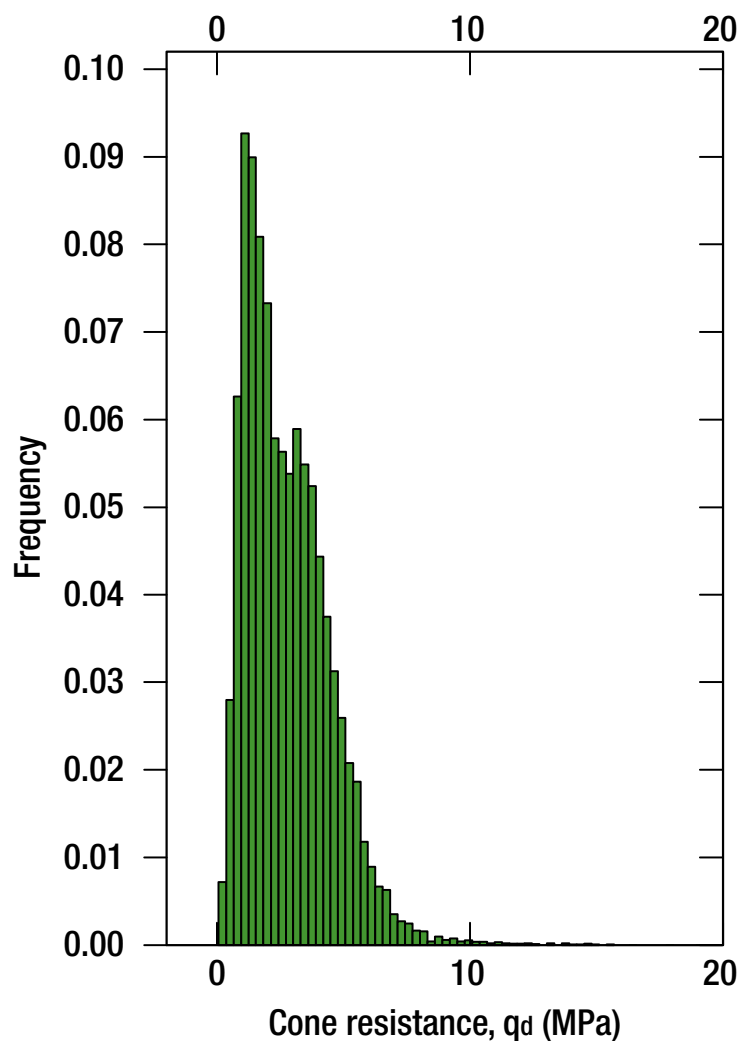
Figure 5. Histogram of q_d values. Full survey grid.
