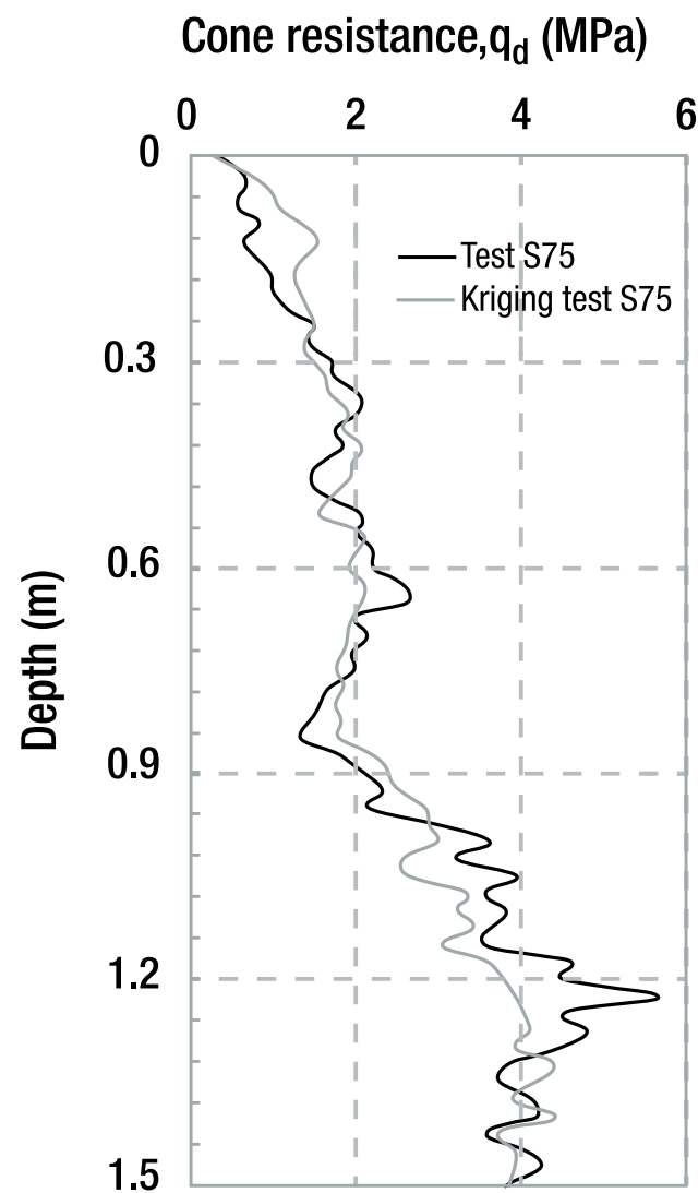
Figure 12. OK estimation of q_d . yz-plane cross-sectional profile. PANDA test 75. Test slab 4.
