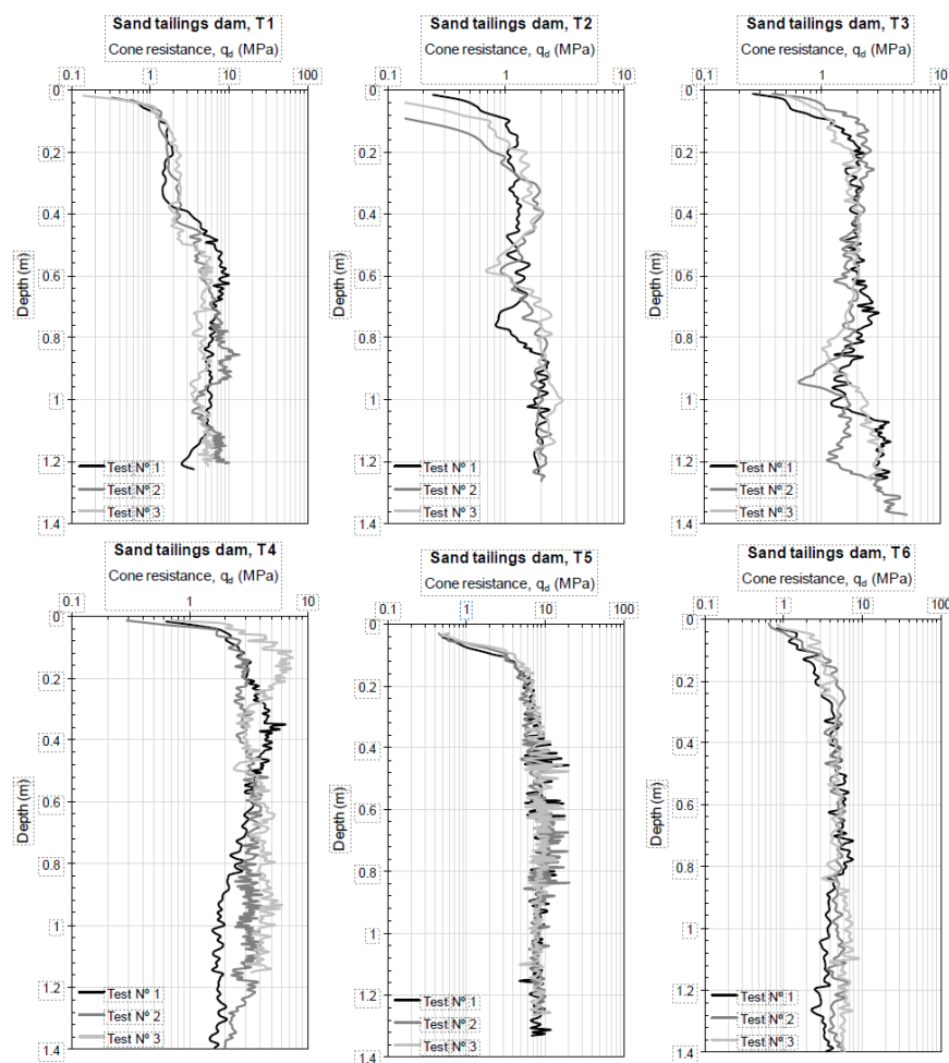
Figure 3. Cone resistance ( q_d ) as a function of depth, measured in 6 Chilean classified sand tailings dams.
