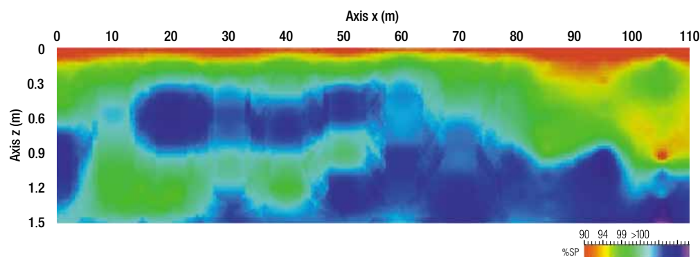
Figure 13. % SP compaction percentages estimated by OK. x-z plane longitudinal profile. Survey grid: second third, near the foot of the embankment.
