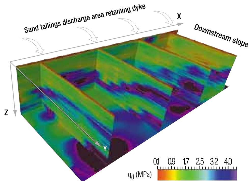
Figure 9. OK estimation of q_d . Full survey grid.
