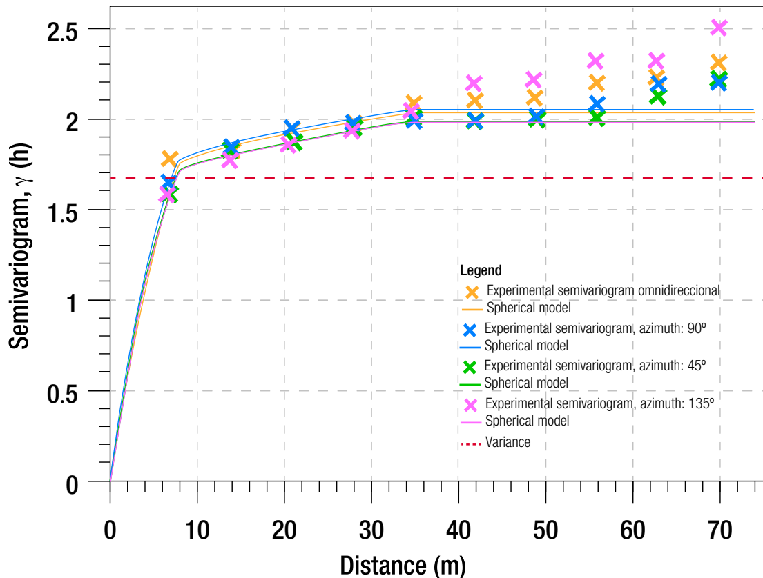
Figure 8. Experimental semivariograms and theoretical models for q_d . Horizontal analysis plane.
