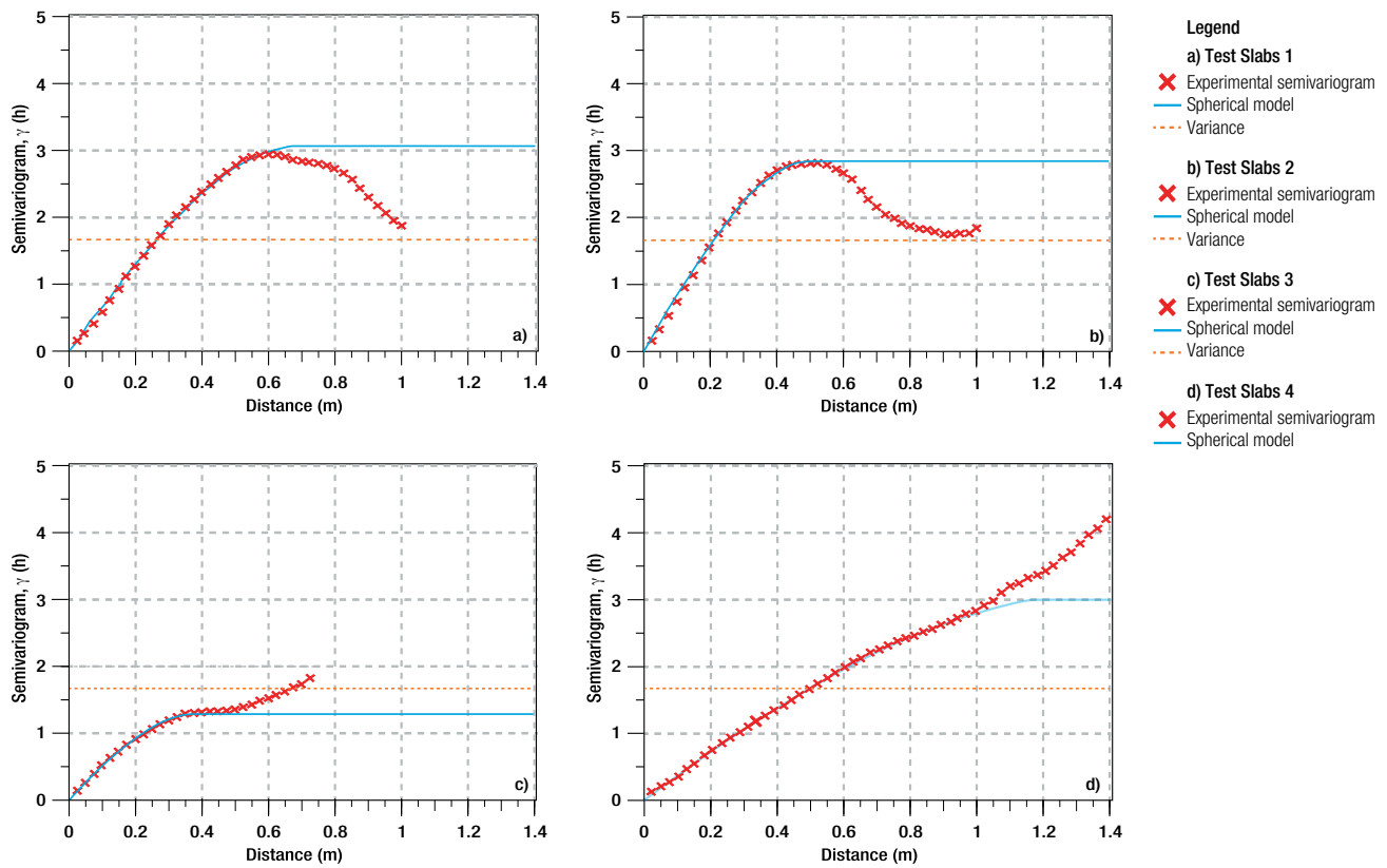
Figure 7. Experimental semivariograms and theoretical models for q_d . Vertical analysis plane.
