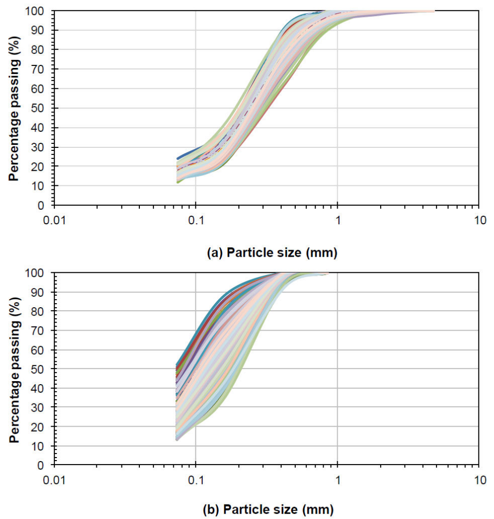
Figure 2. Variation of the particle size distribution (PSD). Operational control of two sand tailings dams of medium copper mining in Chile. (a) Sand tailings T1. (b) Sand tailings T2. (see Table 2).
