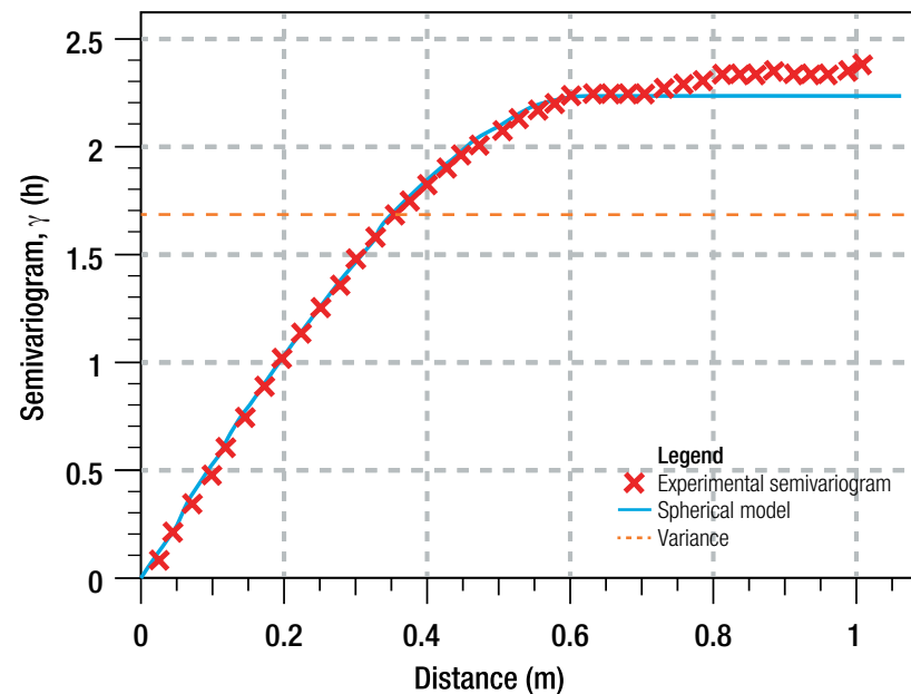
Figure 6. Experimental semivariogram and omnidirectional theoretical model for q_d in the vertical direction. Full survey grid.
