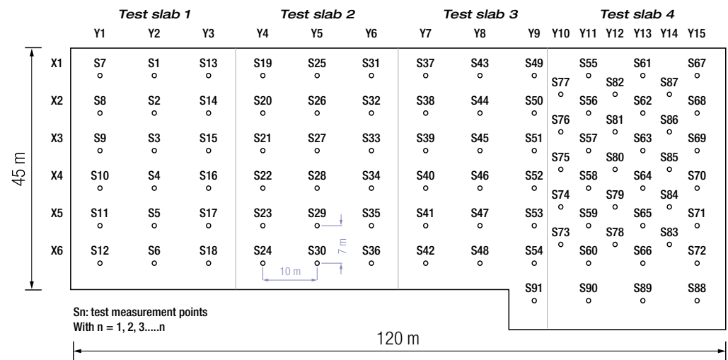
Figure 4. Geometry of the survey grid and PANDA test points. DS slope embankment of classified sand tailings dam T3.
